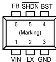
Figure 1. Pin Assignments of FR9204
