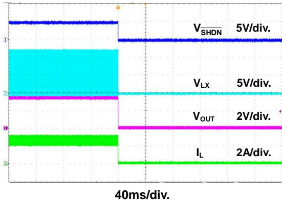
Figure 19. Power Off Through \overline{SHDN} Waveform
