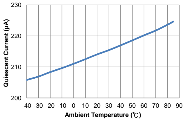
Figure 8. Quiescent Current vs. Ambient Temperature
