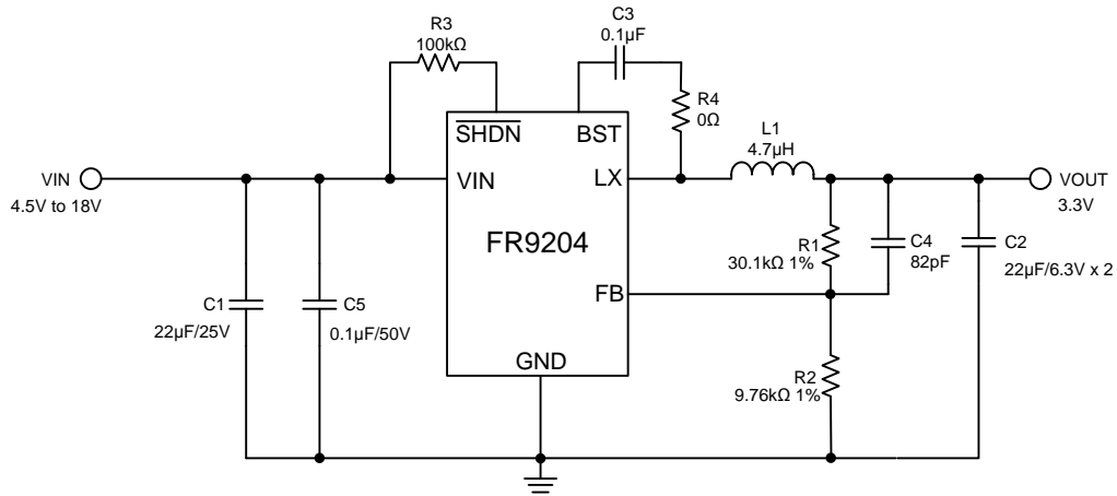
Figure 2. FR9204 Application Circuit
