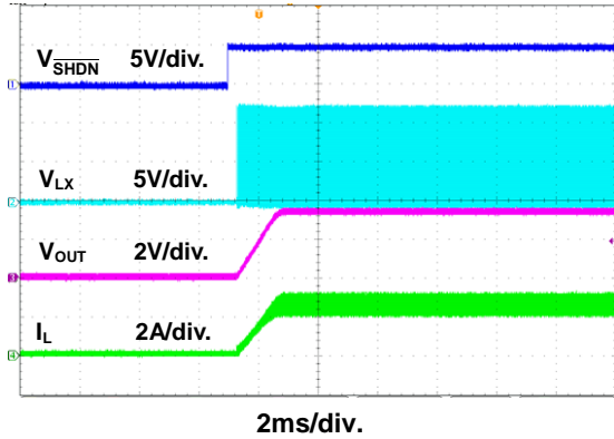
Figure 17. Power On Through \overline{SHDN} Waveform
